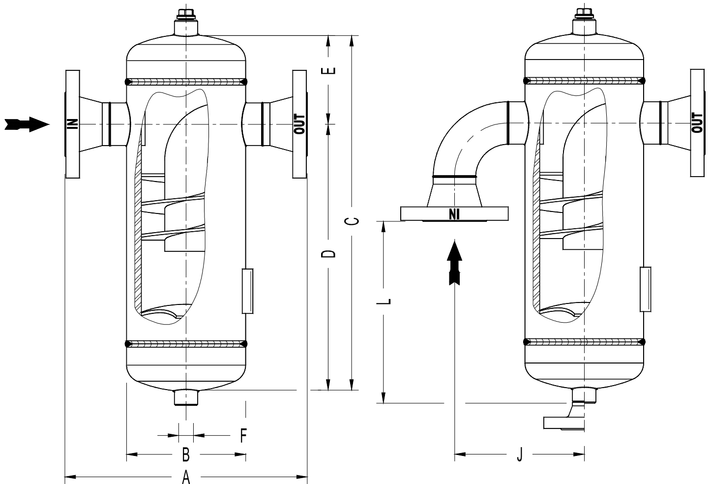
EVH-Elbow vertical inlet / horizontal outlet
