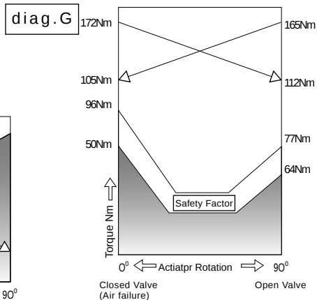
UNBALANCED TORQUE
