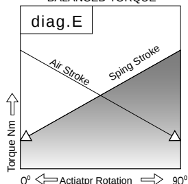
BALANCED TORQUE
