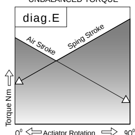
UNBALANCED TORQUE
